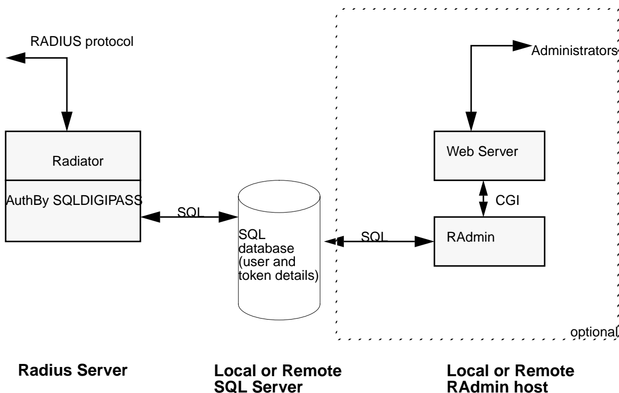
Radiator + RAdmin Digipass architecture
